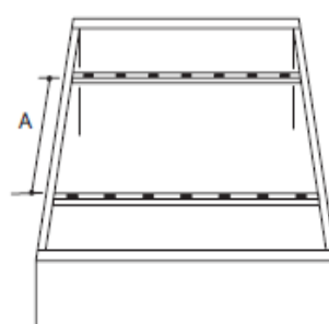
Front to Back Installation 前至后安装
