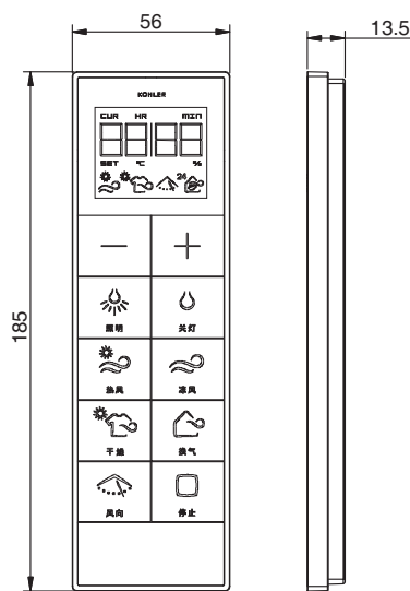
Remote Control 遥控器尺寸图
