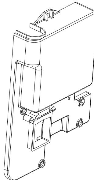
1291994-SP PCBA BOX COVER 电控盒盖
