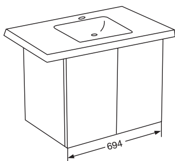
K-72527T—694mm Washbasin Cabinet 脸盆柜 (Not Include Countertop, Washbasin、Legs、Handle) (不含台面、脸盆、支撑脚、拉手)
